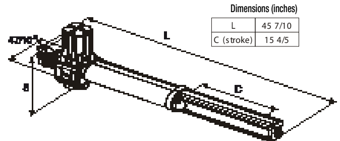
Dimensions (inches)
